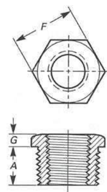
Bussing hexagonal
